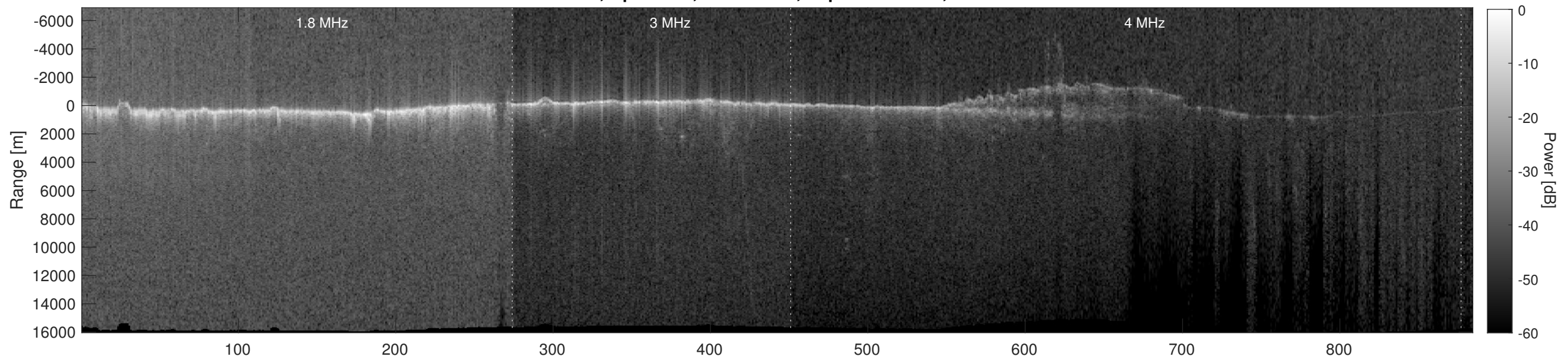
Orbit 7762, Depth-Corrected Cluttergram
