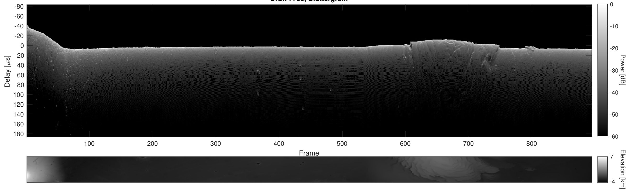
Orbit 7765, Cluttergram
