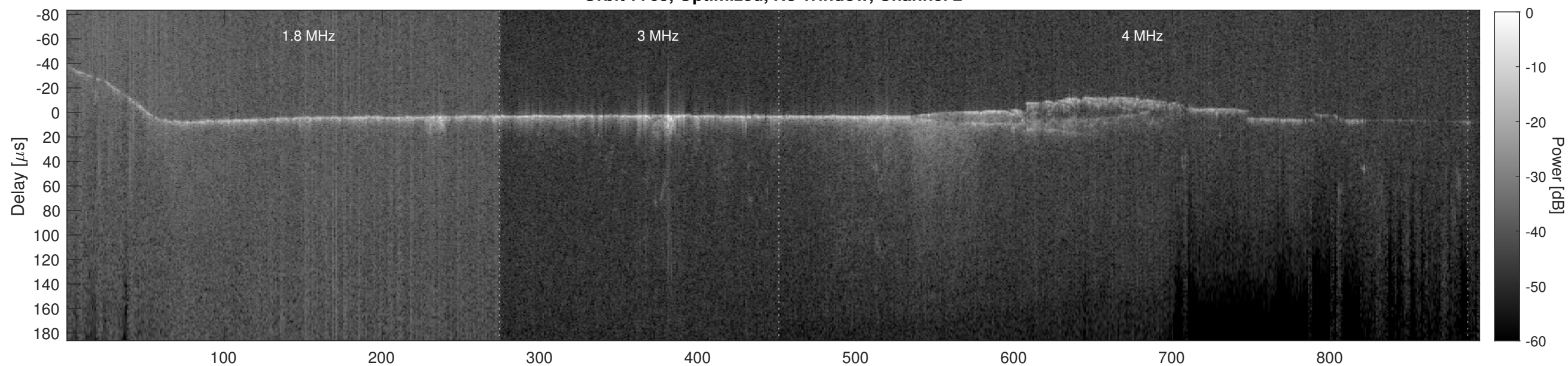
Orbit 7765, Cluttergram
