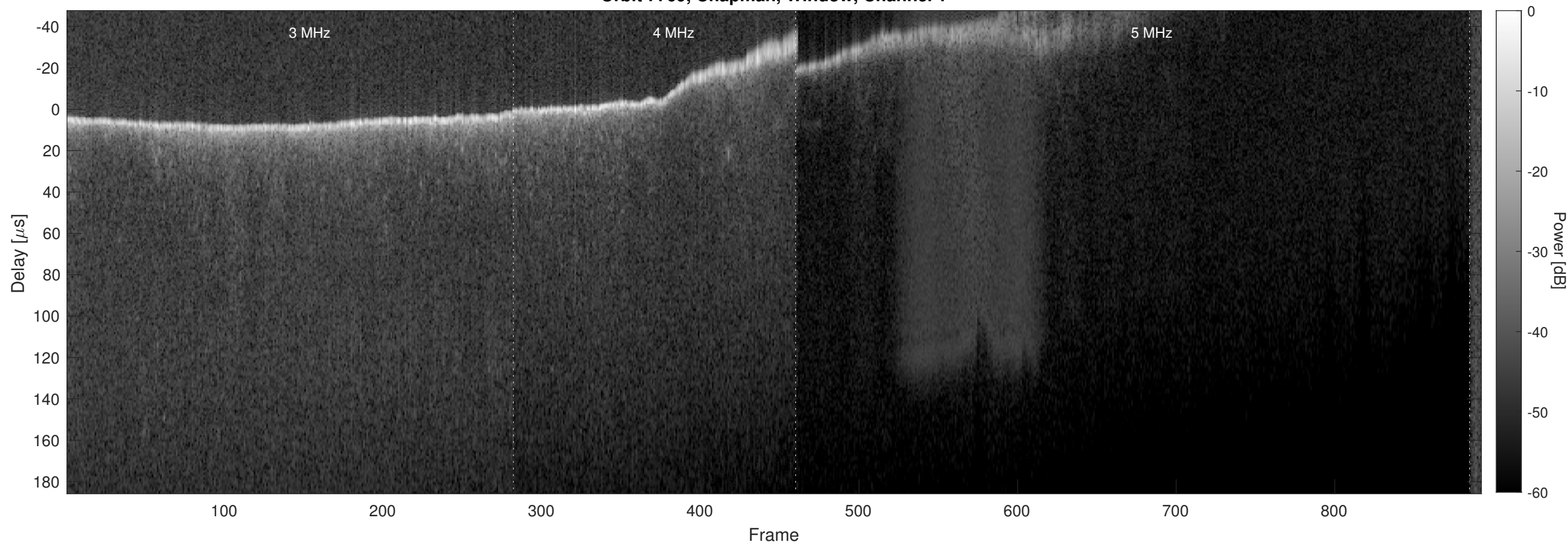
Orbit 7769, Chapman, Window, Channel 2
