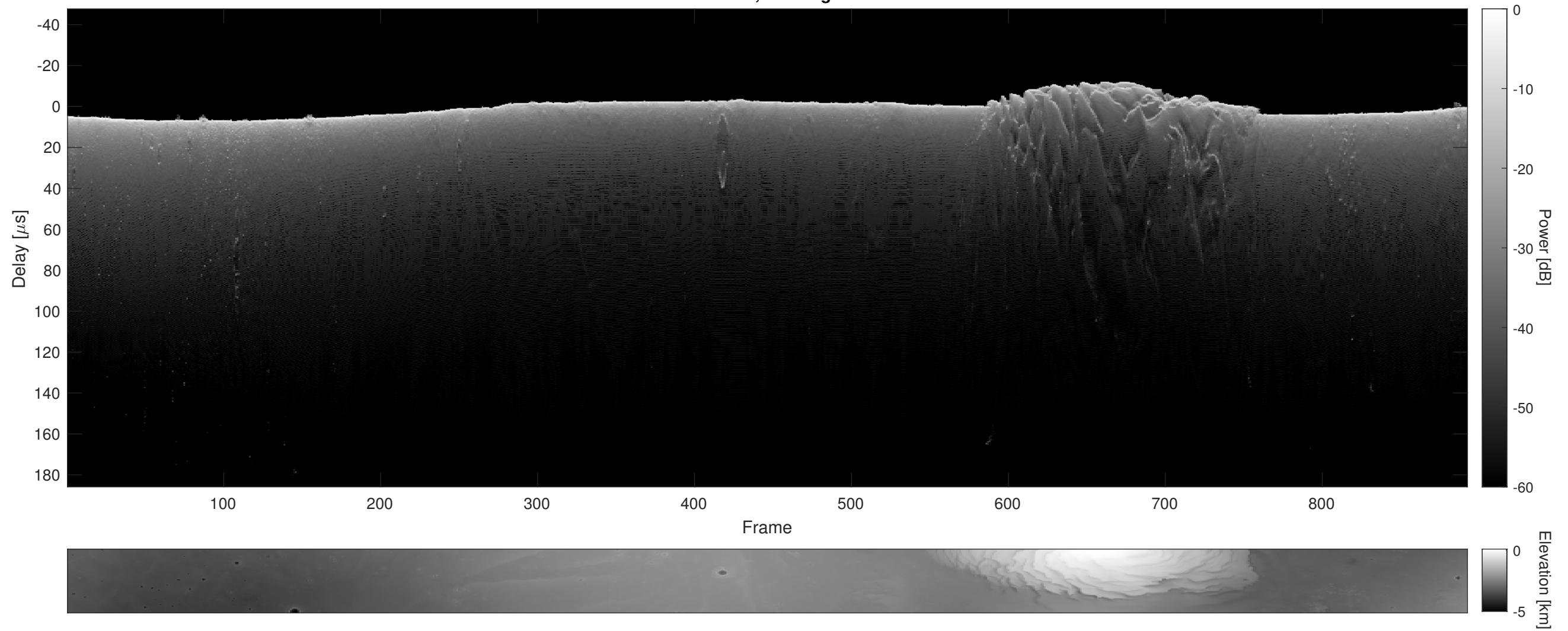
Orbit 7769, Cluttergram
