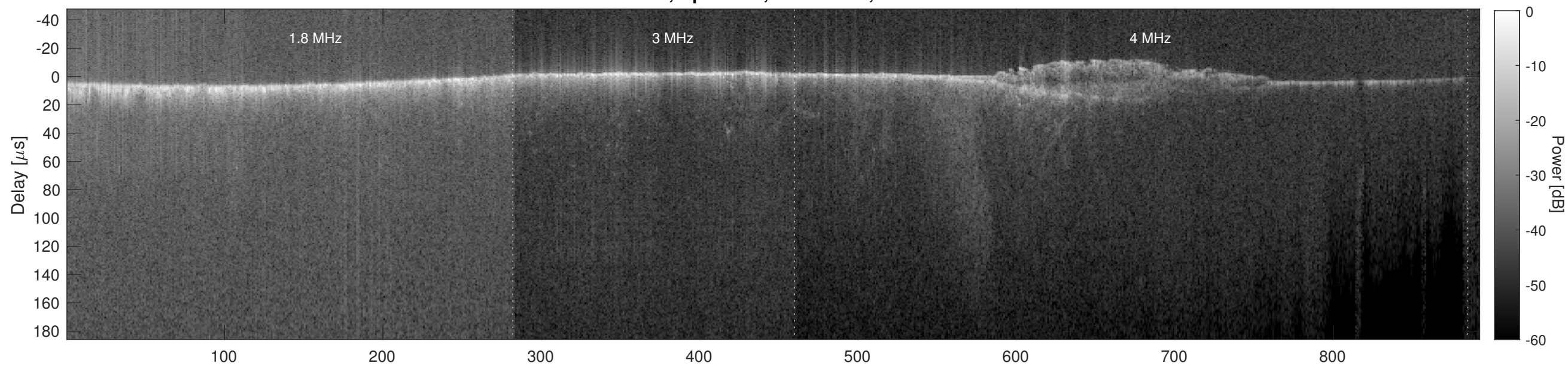
Orbit 7769, Cluttergram
