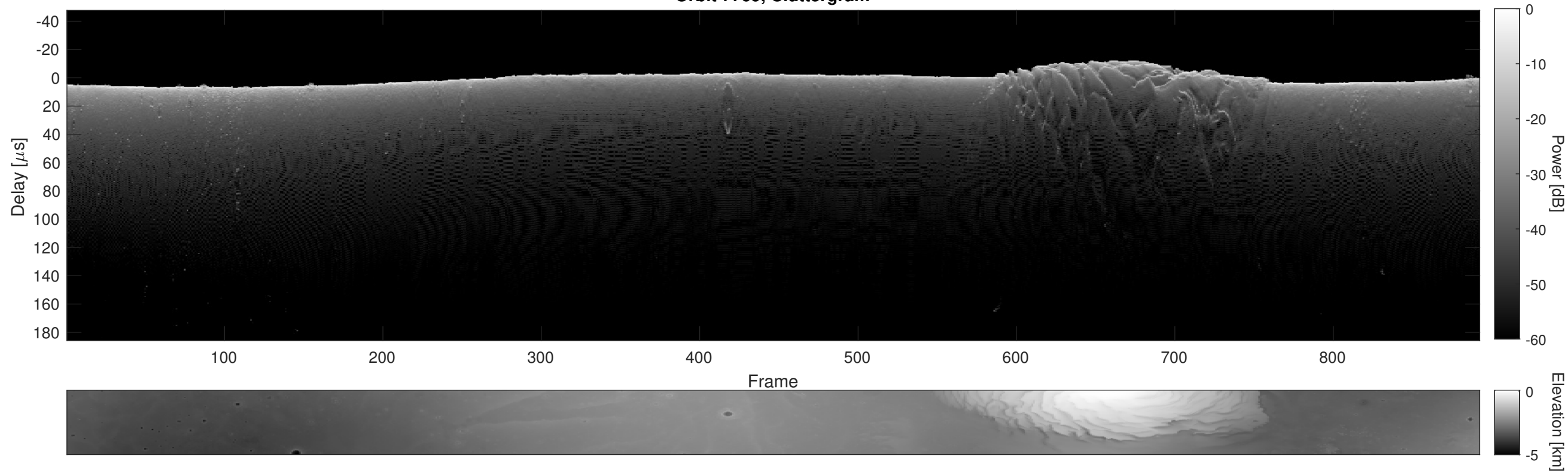
Orbit 7769, Cluttergram
