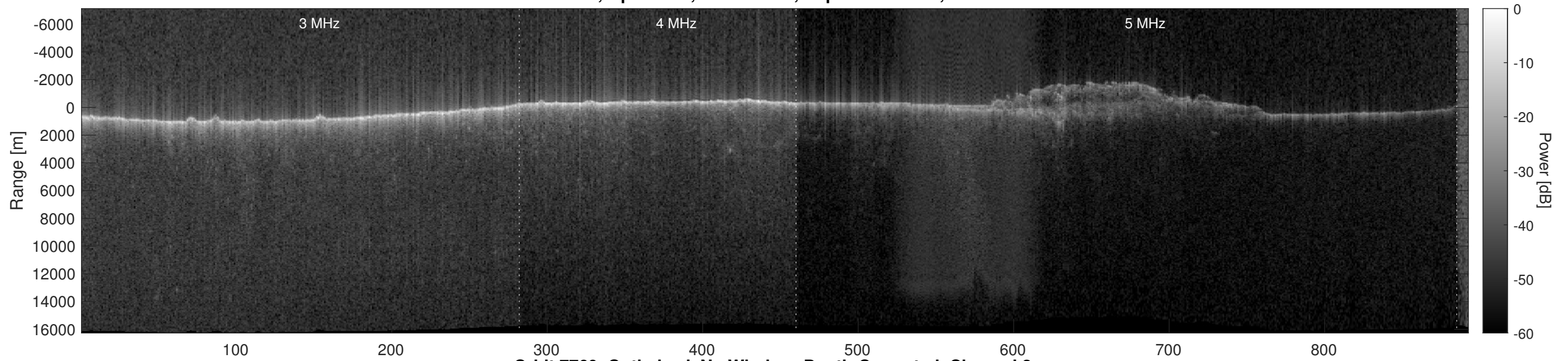
Orbit 7769, Optimized, No Window, Depth-Corrected, Channel 2
