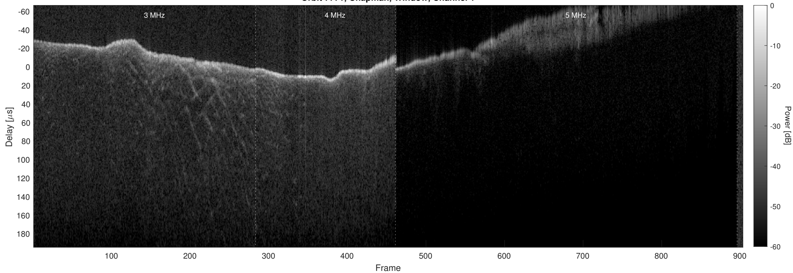
Orbit 7771, Chapman, Window, Channel 2
