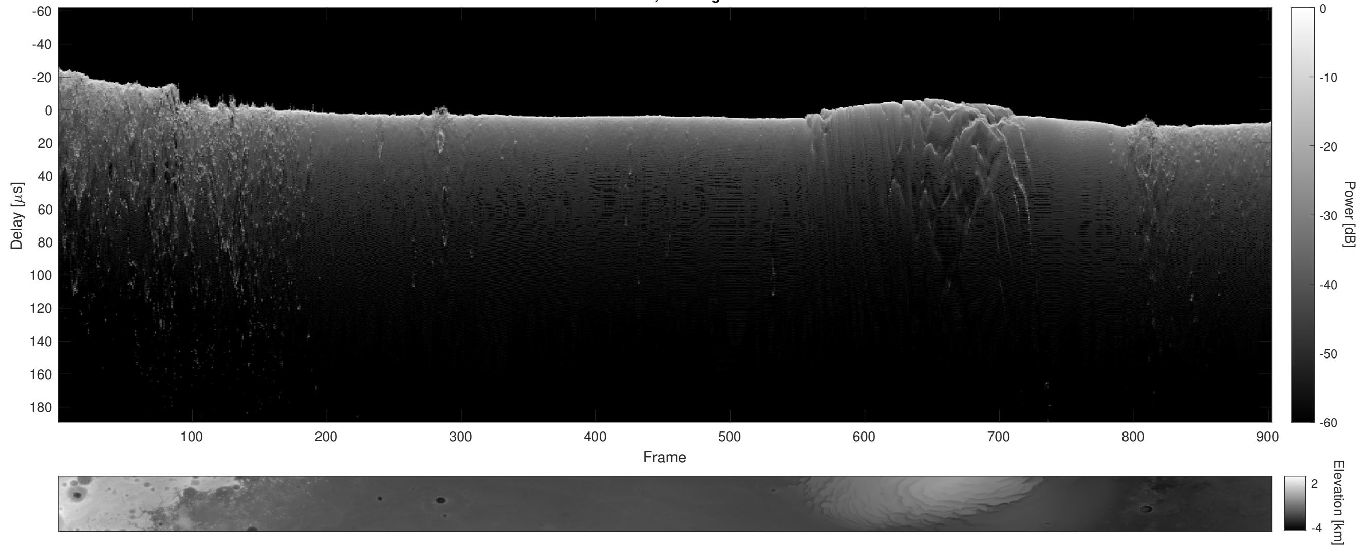
Orbit 7773, Cluttergram
