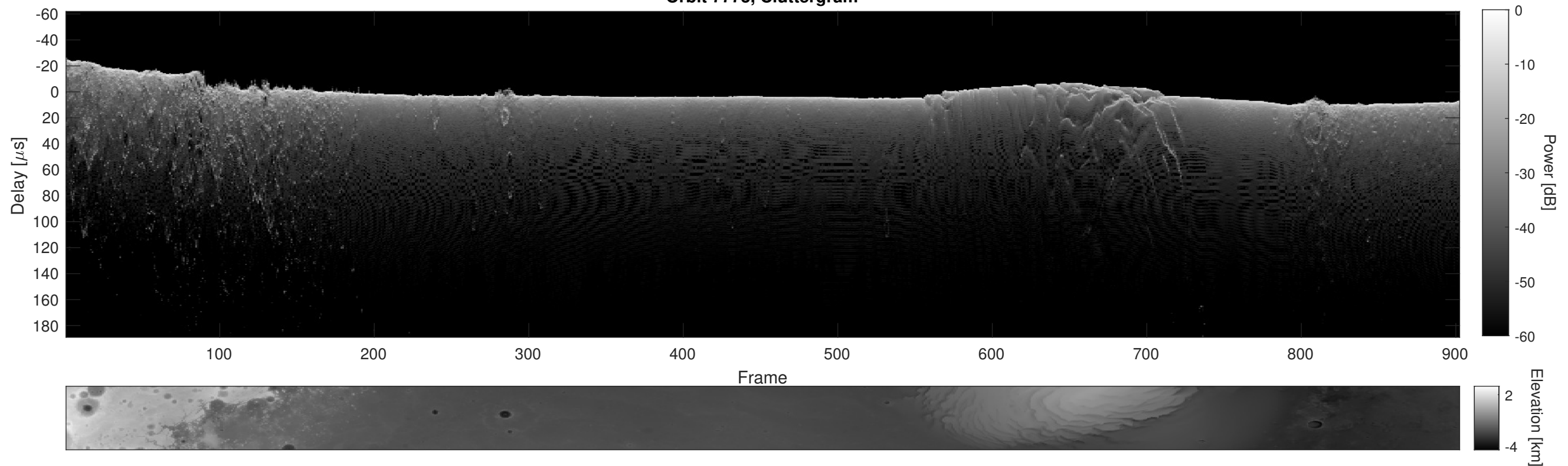
Orbit 7773, Cluttergram
