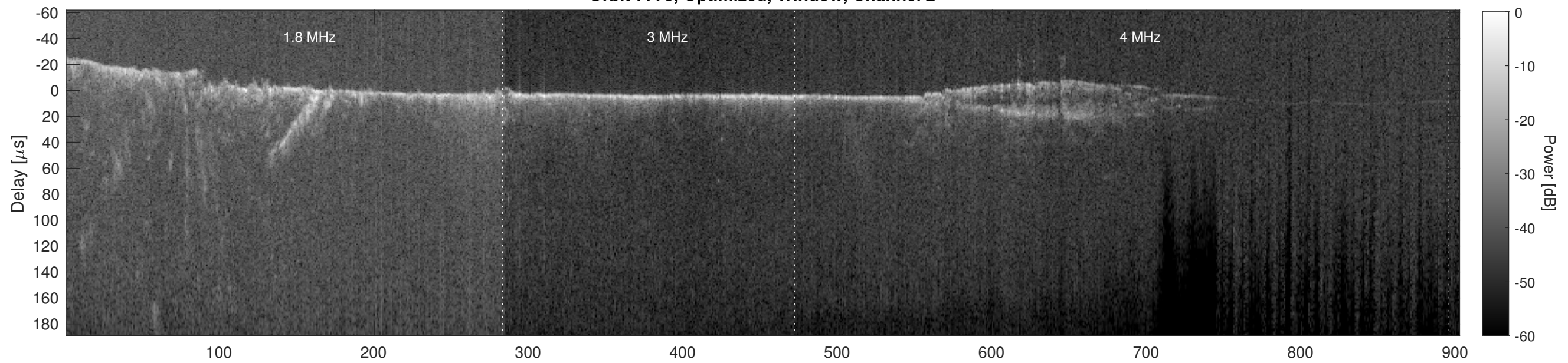
Orbit 7773, Cluttergram
