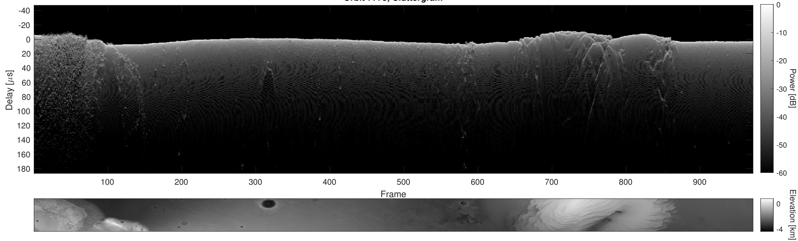
Orbit 7775, Cluttergram
