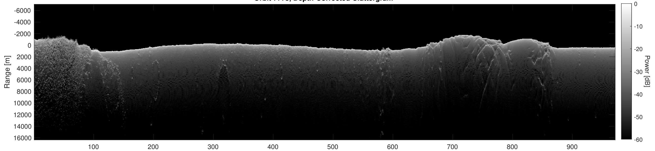
Orbit 7775, Depth-Corrected Cluttergram
