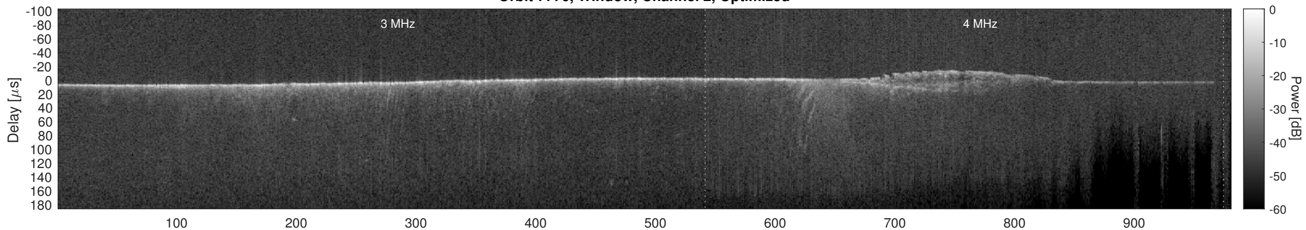
Orbit 7776, Cluttergram
