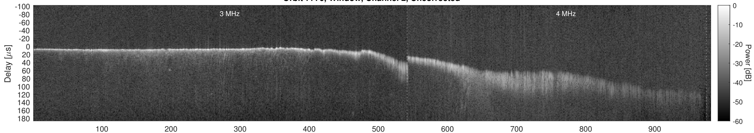
Orbit 7776, Window, Channel 2, Chapman
