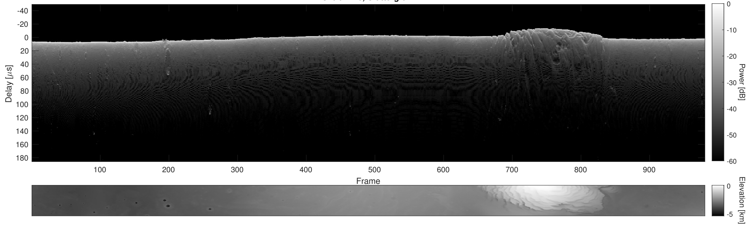
Orbit 7776, Cluttergram
