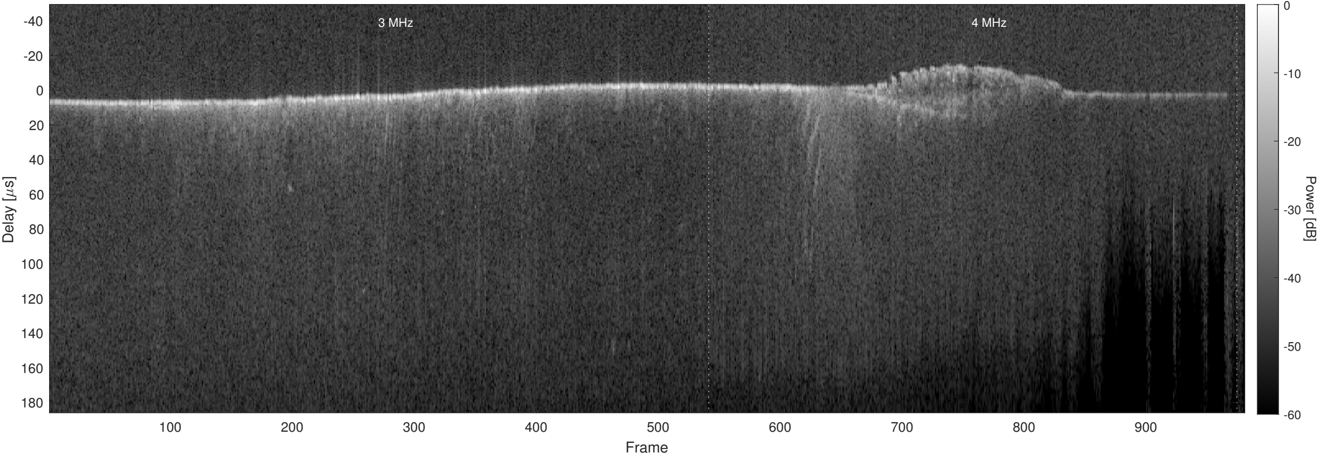
Orbit 7776, Optimized, Window, Channel 2
