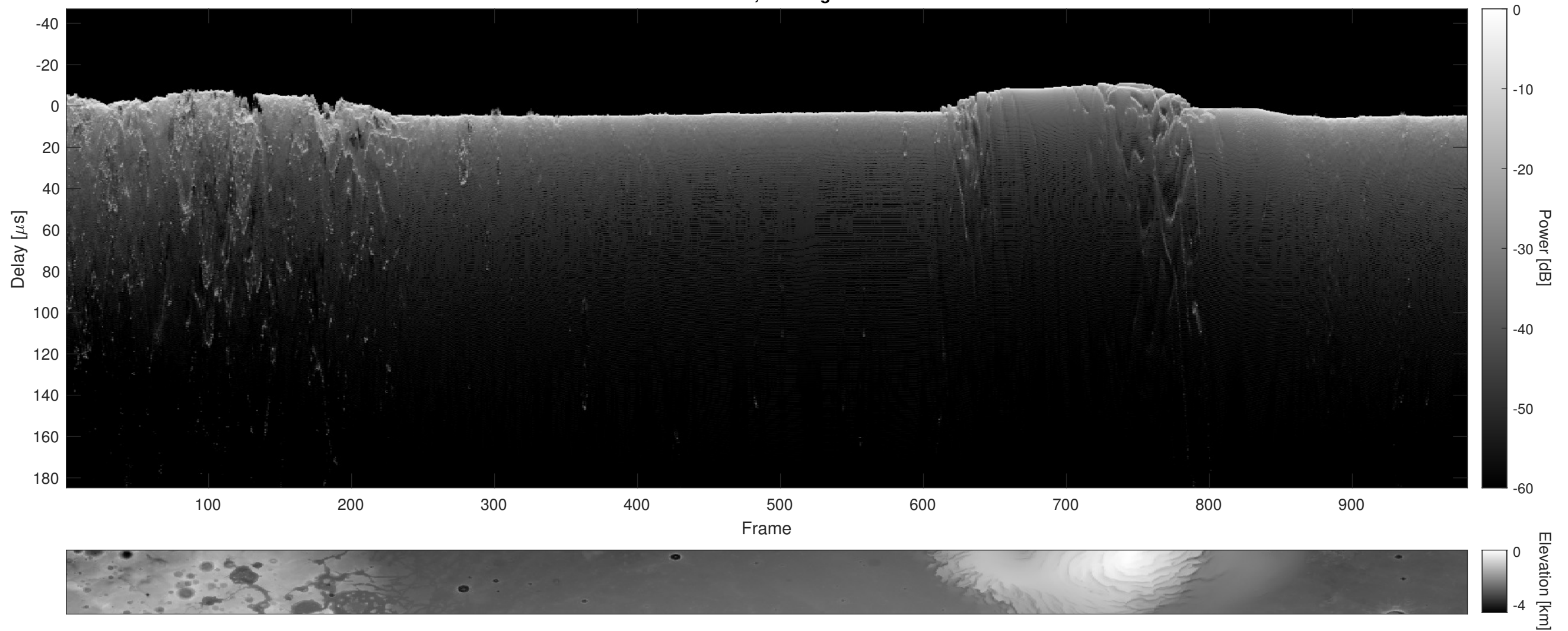
Orbit 7777, Cluttergram
