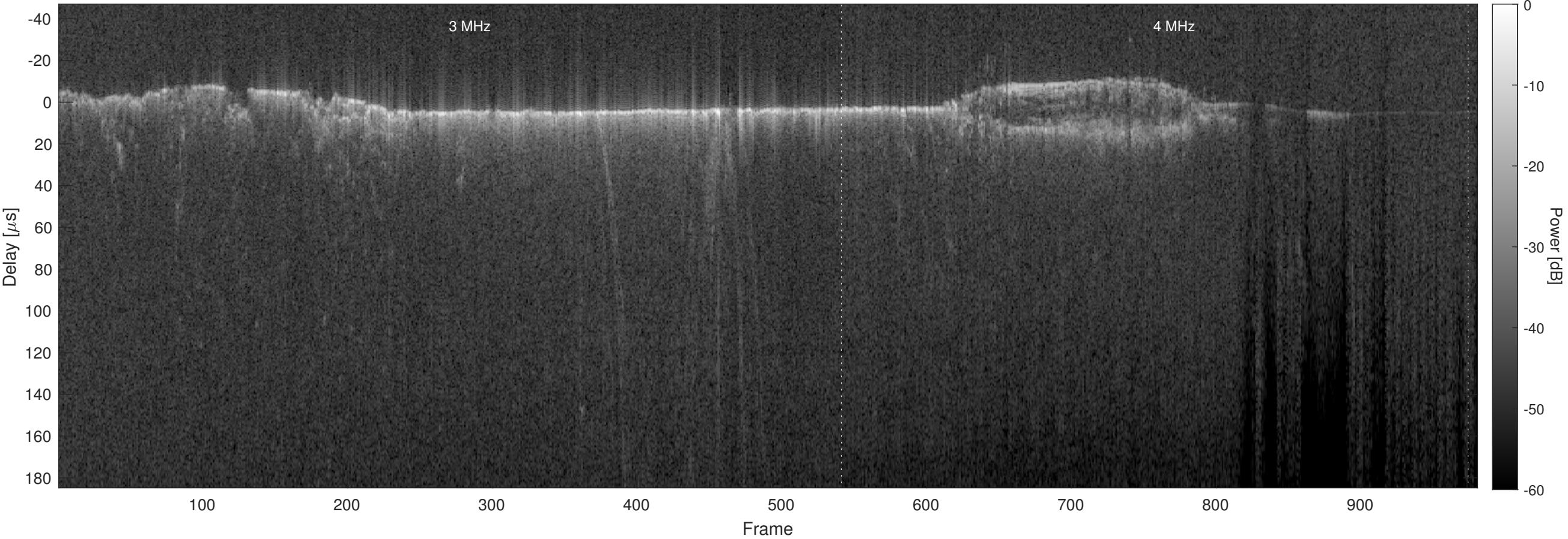
Orbit 7777, Optimized, No Window, Channel 2
