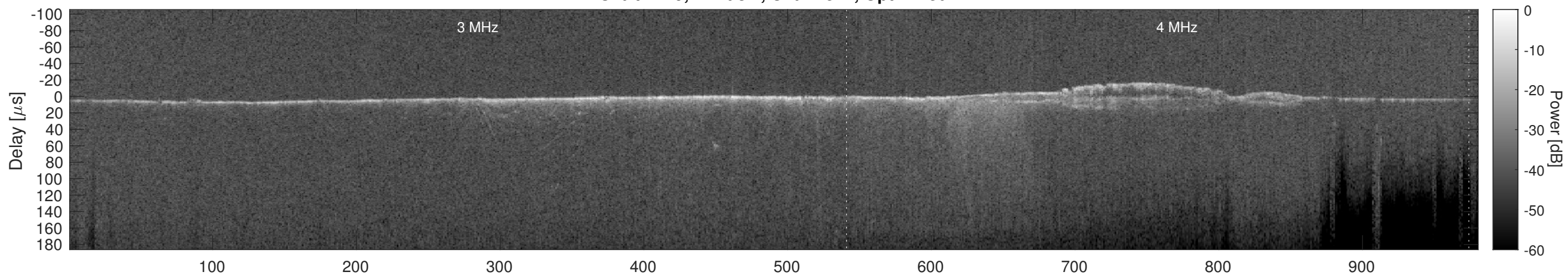
Orbit 7779, Cluttergram
