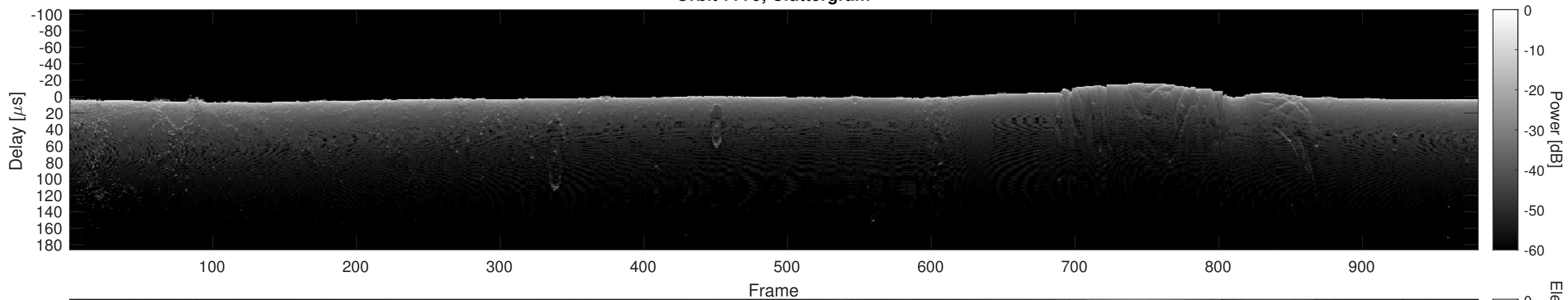
Orbit 7779, Cluttergram
