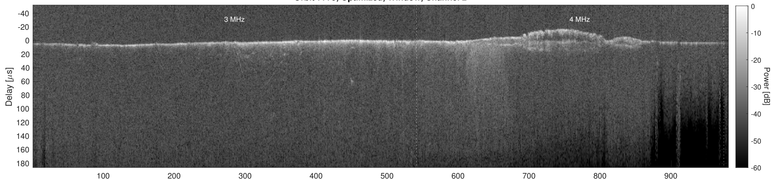
Orbit 7779, Cluttergram
