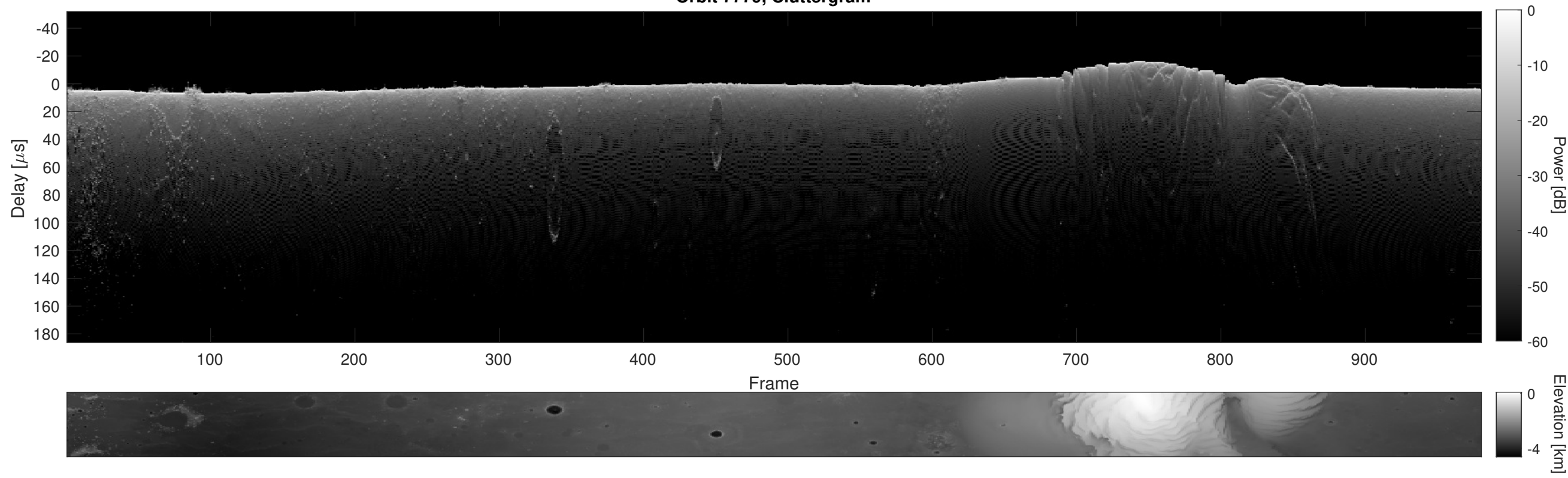
Orbit 7779, Cluttergram
