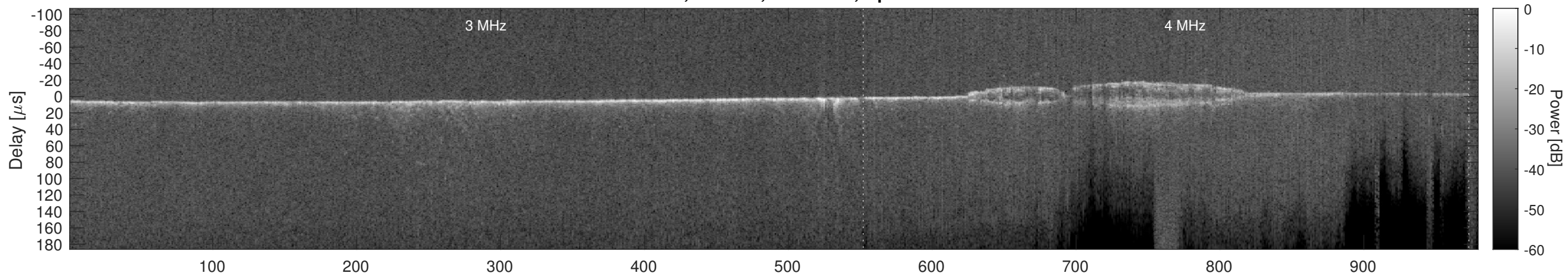
Orbit 7781, Cluttergram
