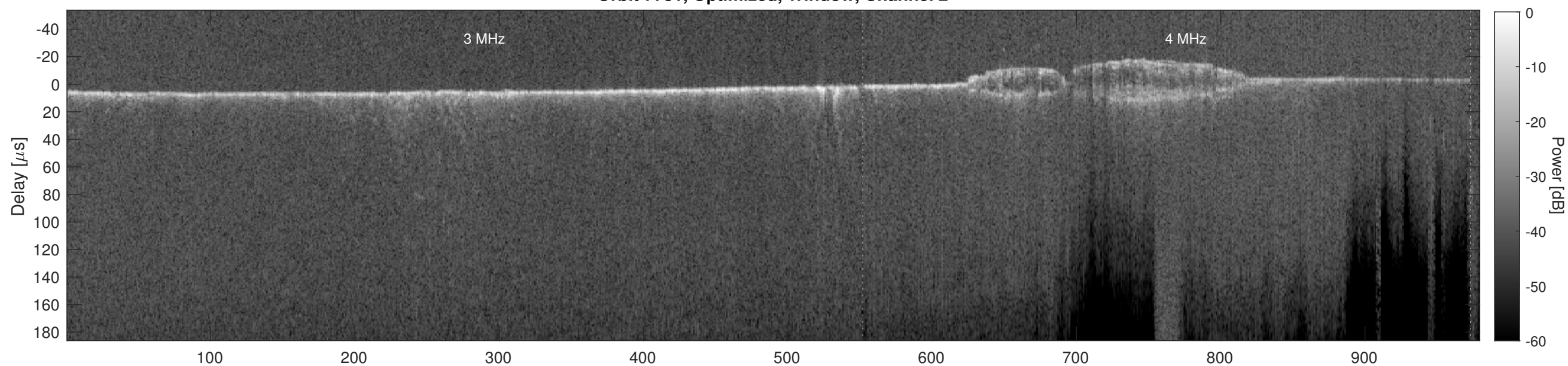
Orbit 7781, Cluttergram
