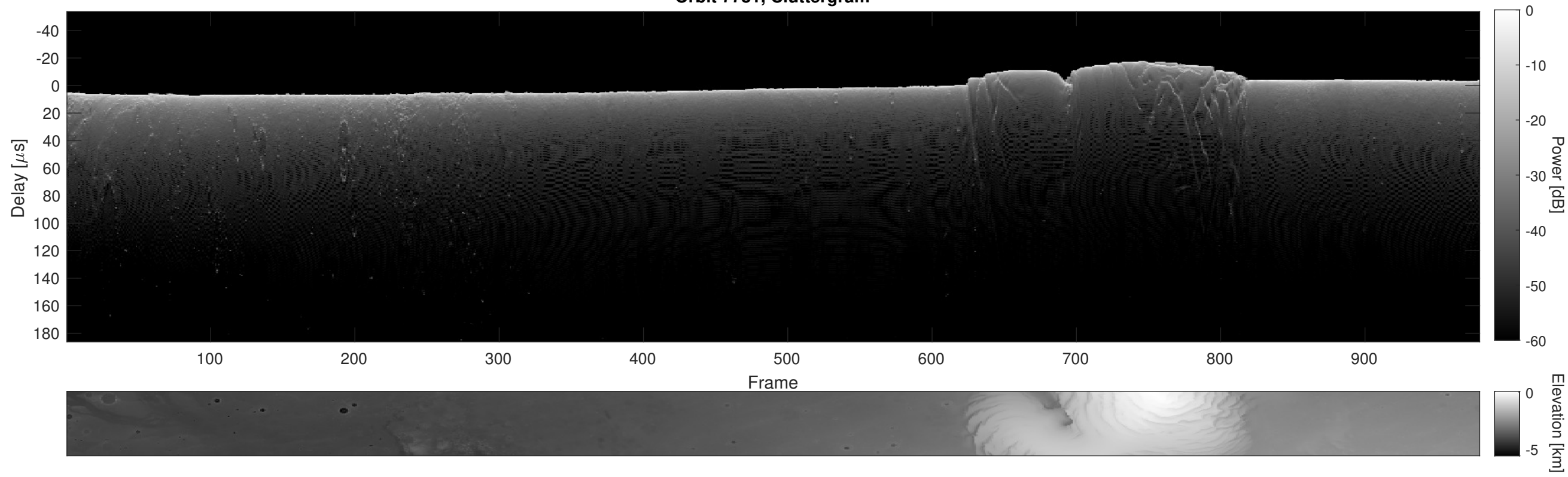
Orbit 7781, Cluttergram
