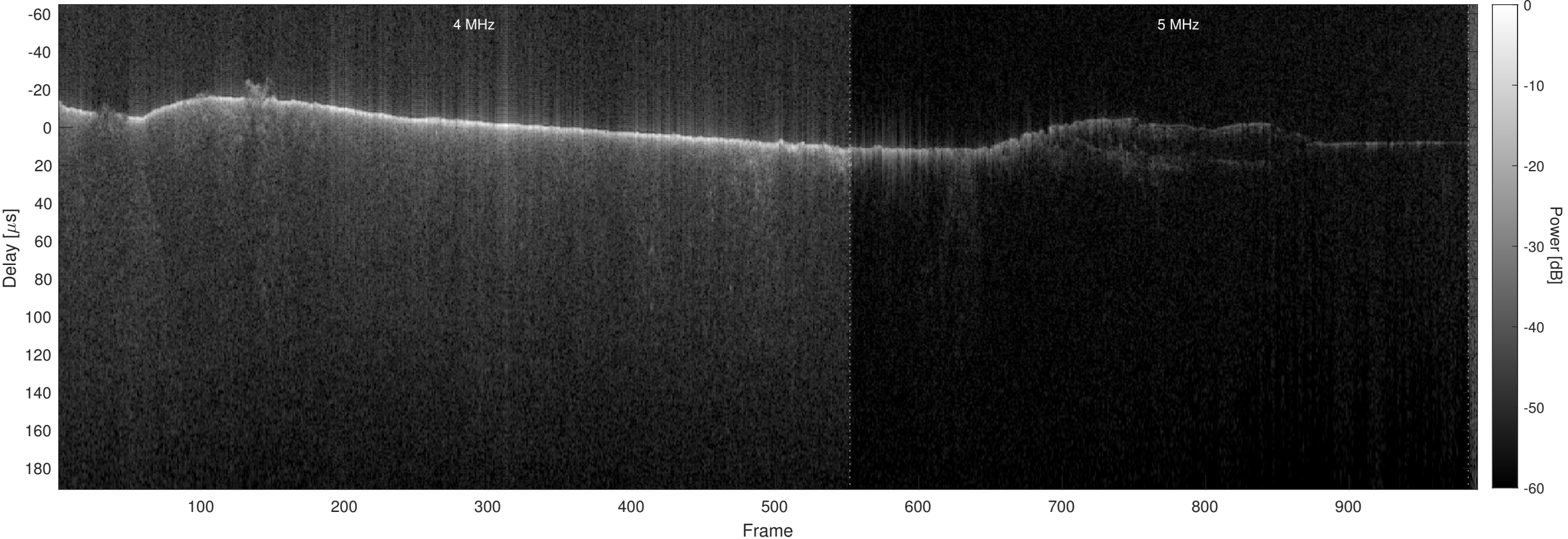
Orbit 7782, Optimized, No Window, Channel 2
