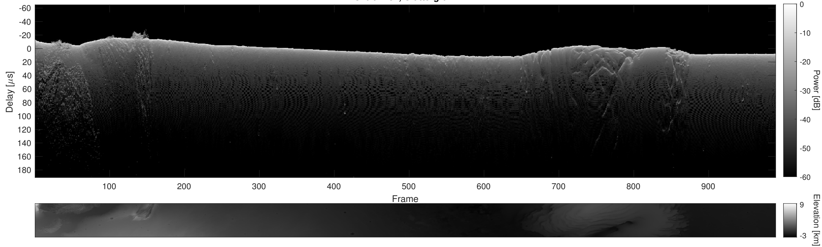
Orbit 7782, Cluttergram
