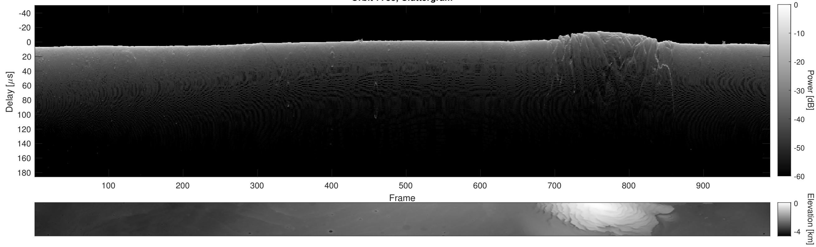
Orbit 7783, Cluttergram
