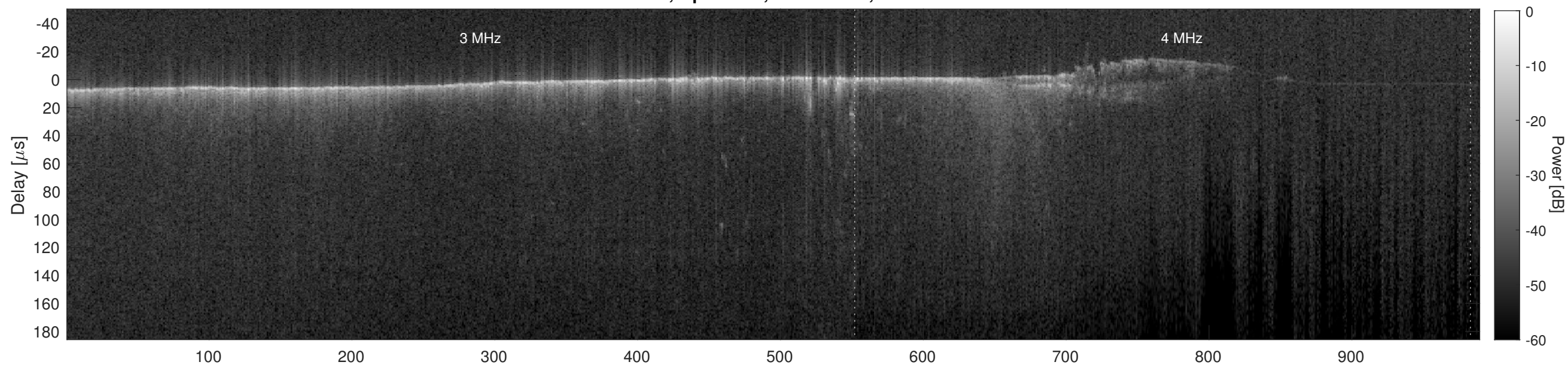
Orbit 7783, Cluttergram
