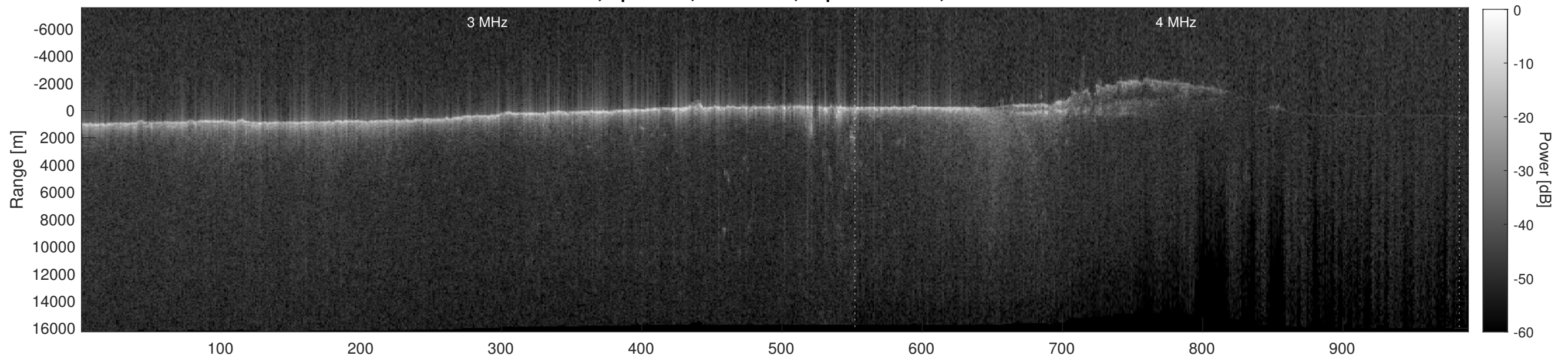
Orbit 7783, Depth-Corrected Cluttergram
