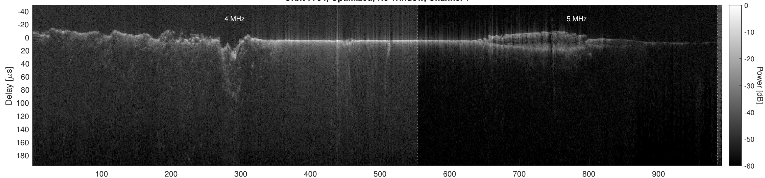
Orbit 7784, Optimized, No Window, Channel 2
