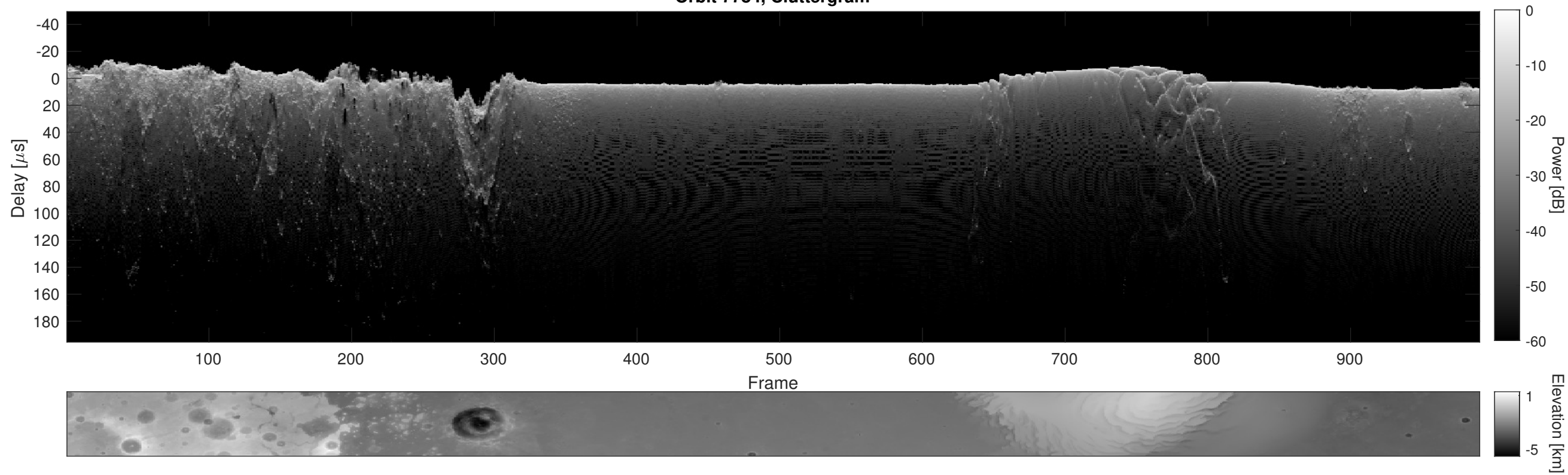
Orbit 7784, Cluttergram
