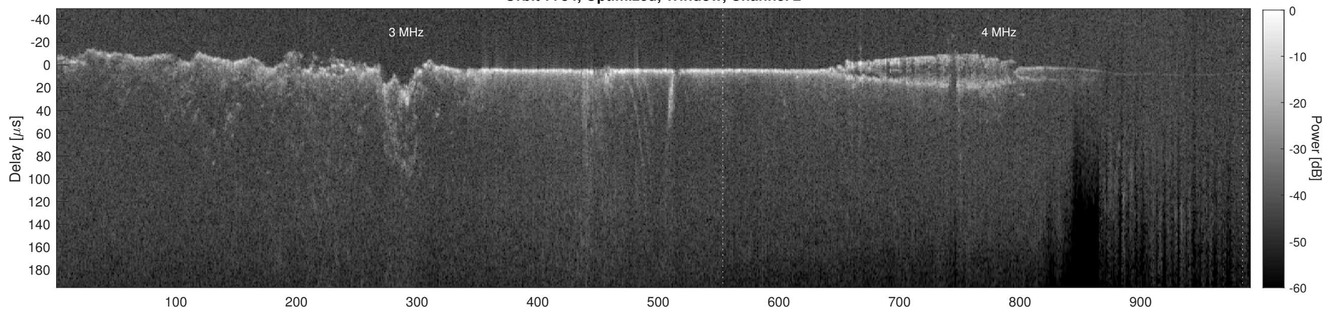
Orbit 7784, Cluttergram
