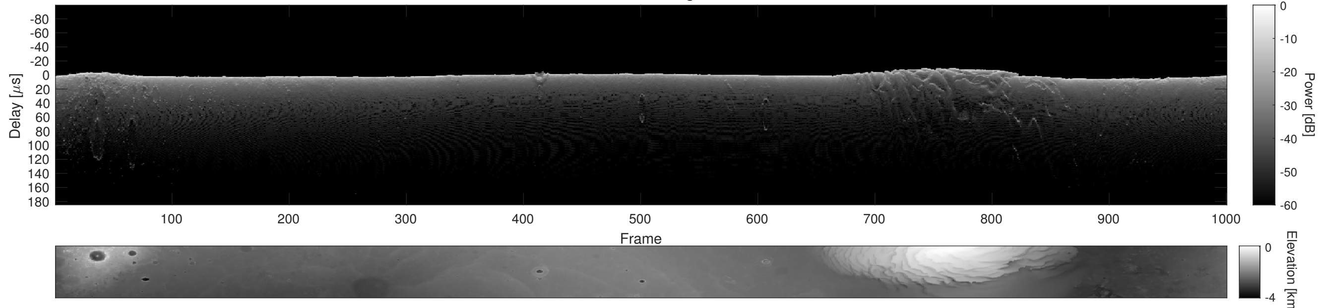
Orbit 7787, Cluttergram
