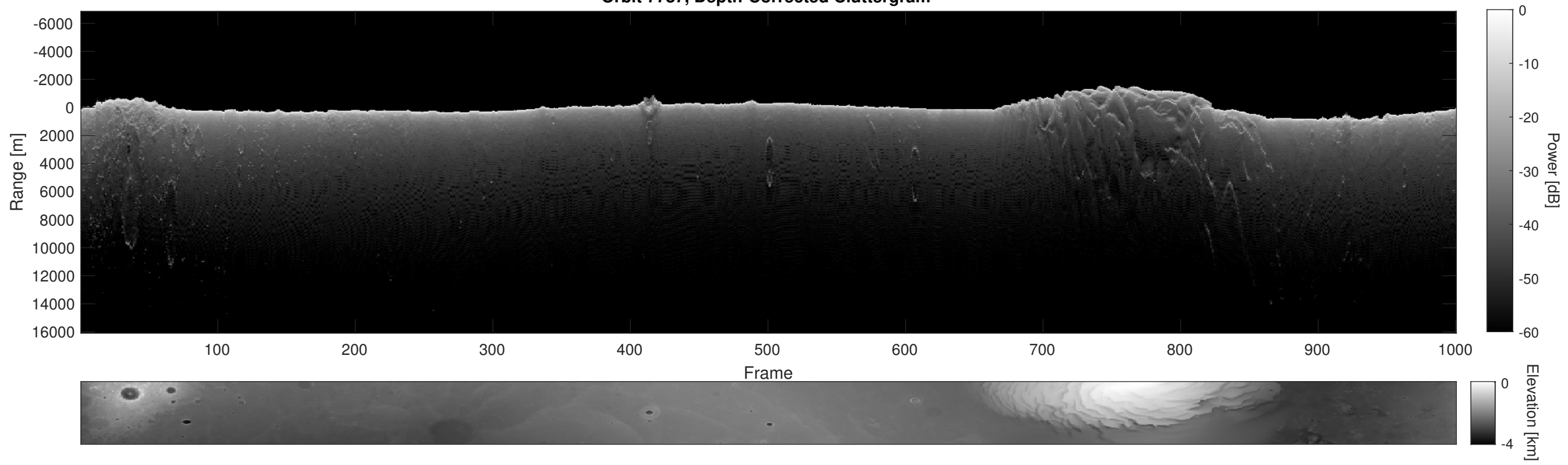
Orbit 7787, Depth-Corrected Cluttergram
