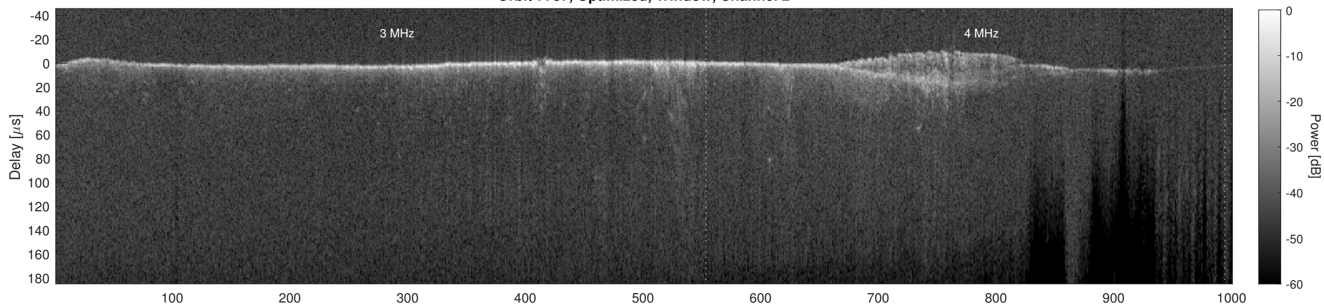
Orbit 7787, Cluttergram
