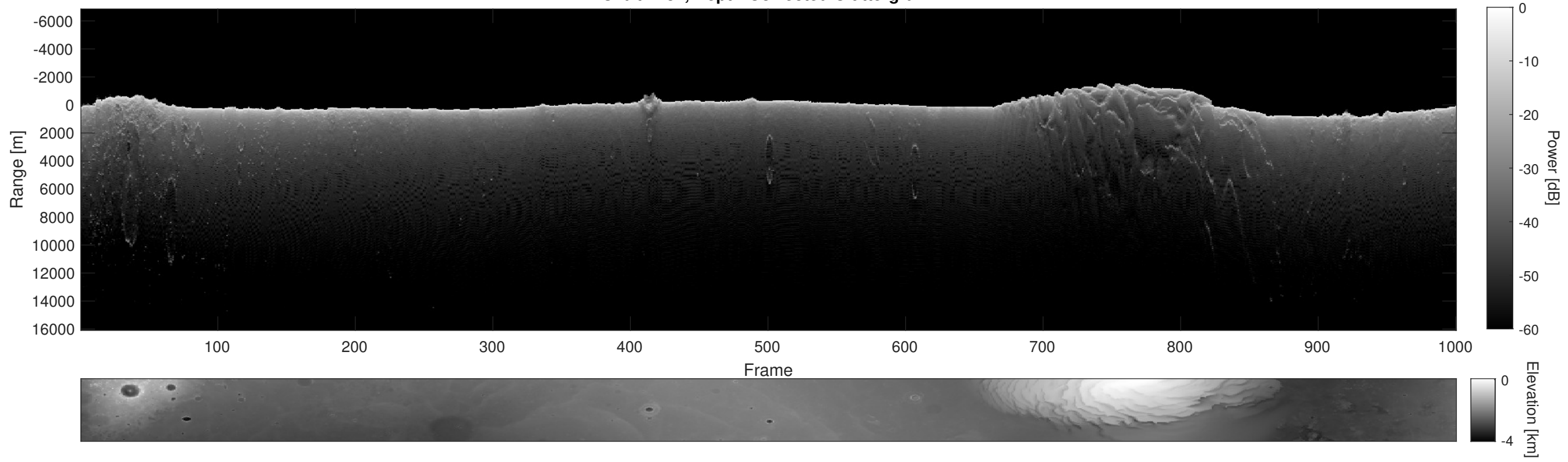
Orbit 7787, Depth-Corrected Cluttergram
