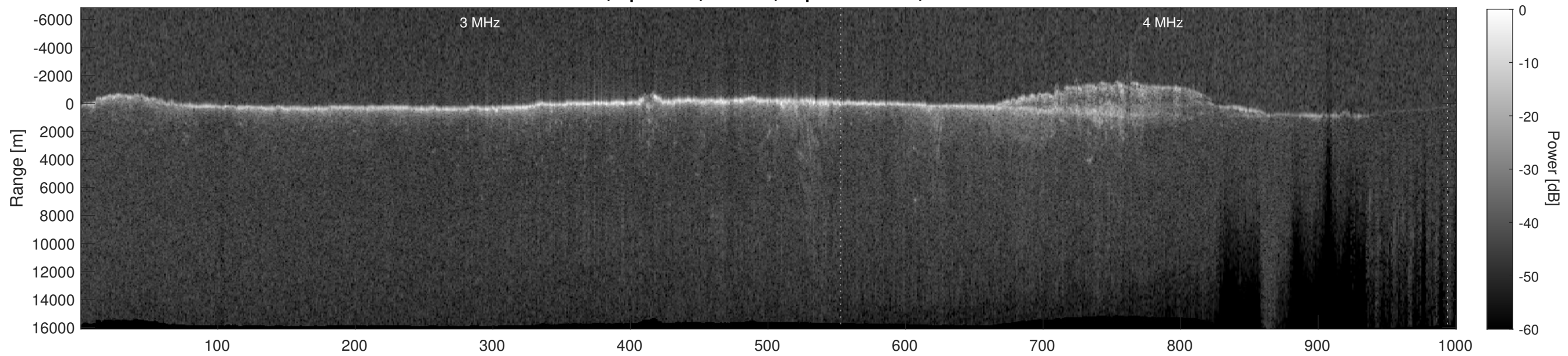
Orbit 7787, Depth-Corrected Cluttergram
