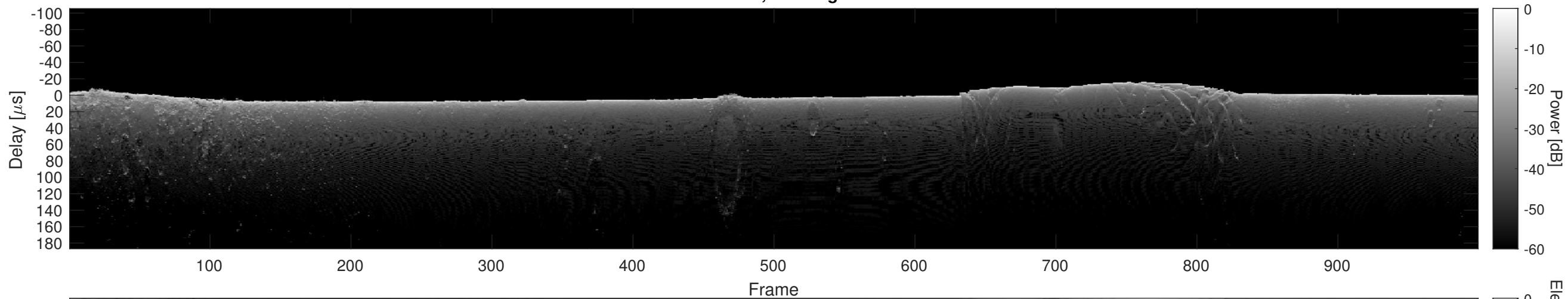
Orbit 7788, Cluttergram
