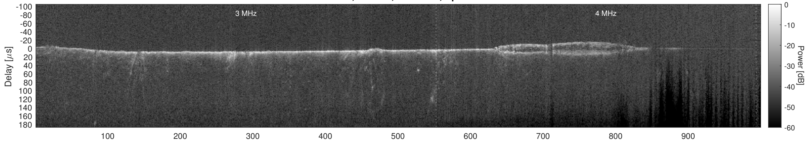
Orbit 7788, Cluttergram
