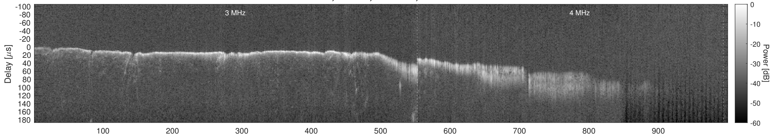
Orbit 7788, Window, Channel 2, Chapman
