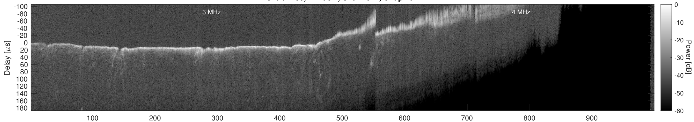
Orbit 7788, Window, Channel 2, Optimized
