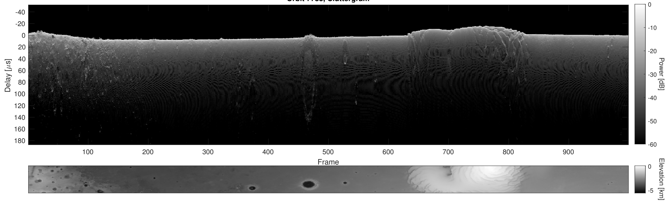
Orbit 7788, Cluttergram
