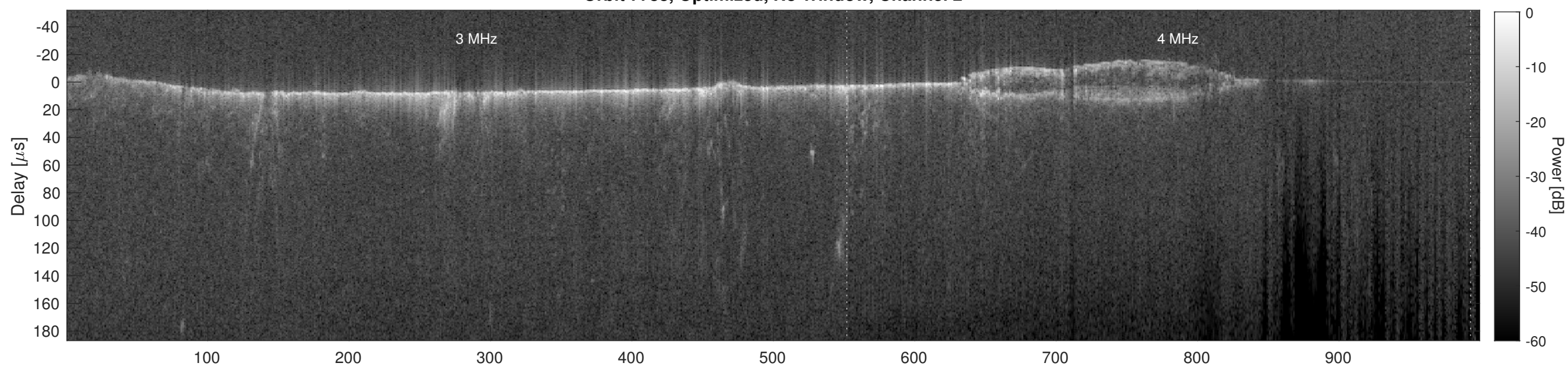
Orbit 7788, Cluttergram
