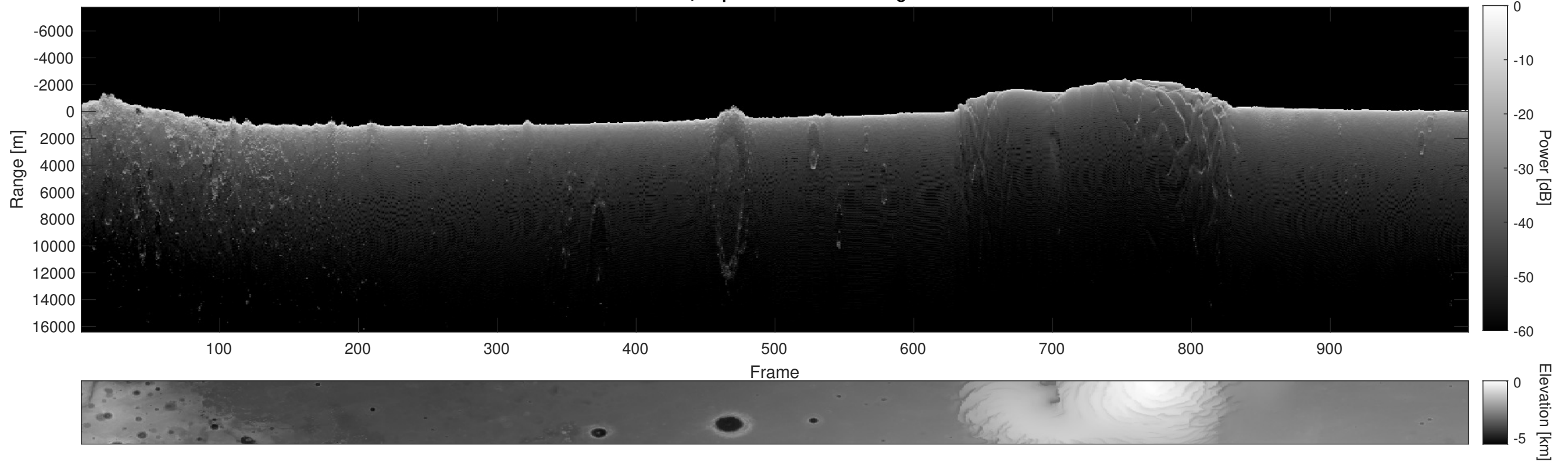
Orbit 7788, Depth-Corrected Cluttergram
