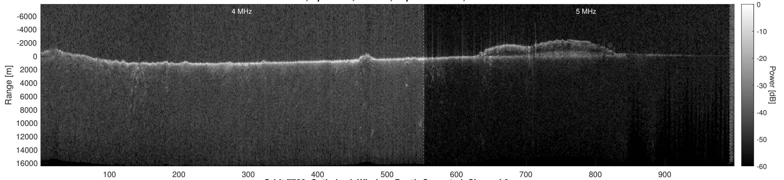
Orbit 7788, Optimized, Window, Depth-Corrected, Channel 2
