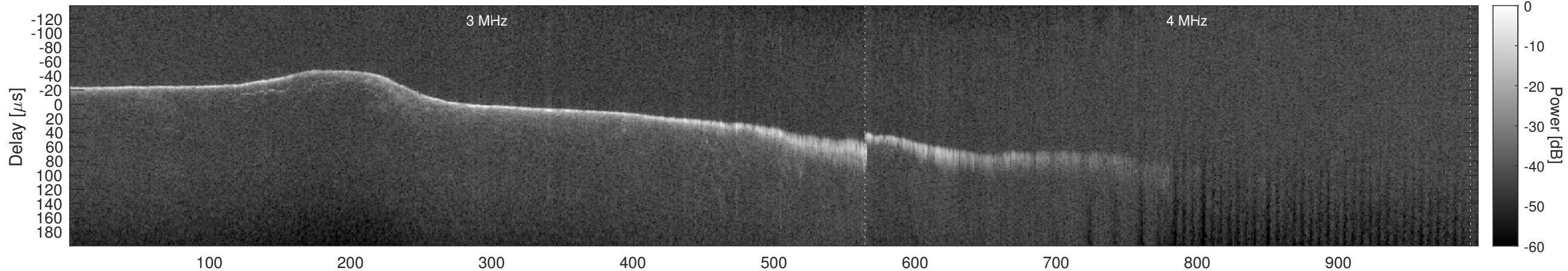
Orbit 7789, Window, Channel 2, Chapman
