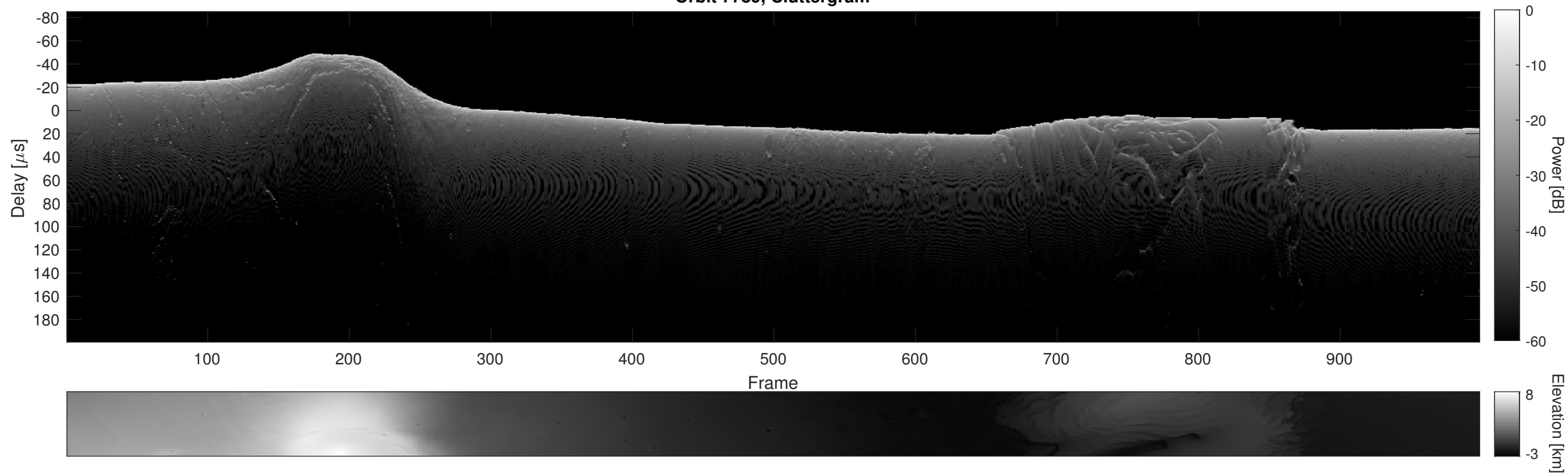
Orbit 7789, Cluttergram
