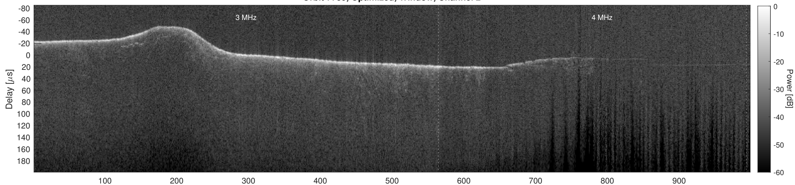
Orbit 7789, Cluttergram
