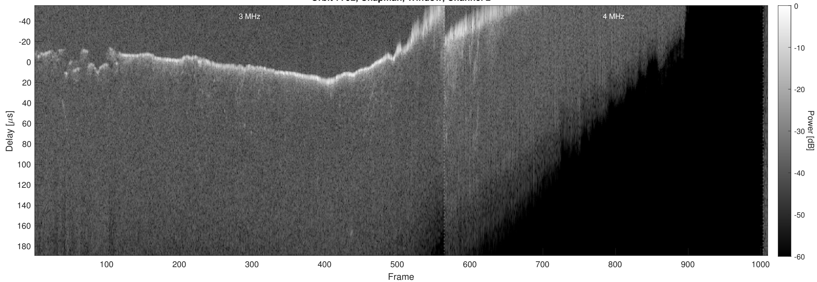
Orbit 7792, Chapman, Window, Channel 2
