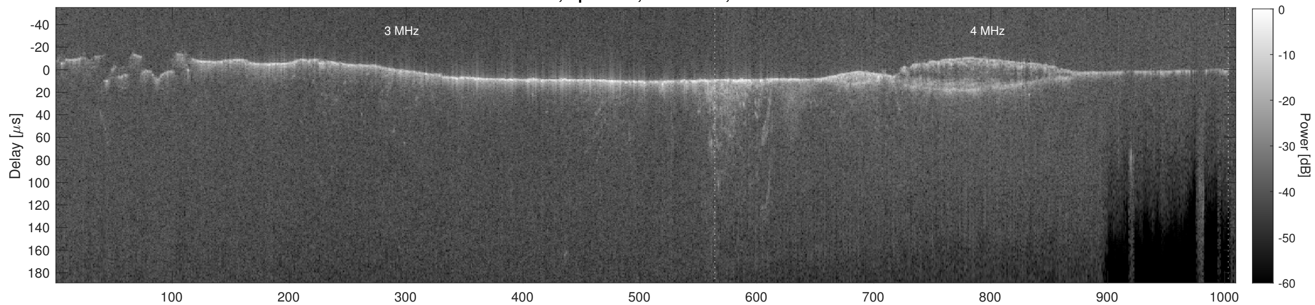
Orbit 7792, Cluttergram
