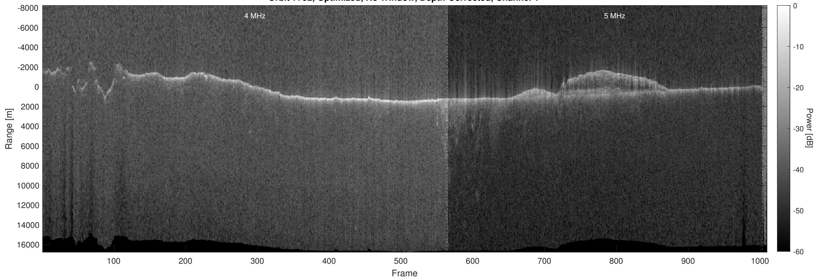
Orbit 7792, Optimized, No Window, Depth-Corrected, Channel 2
