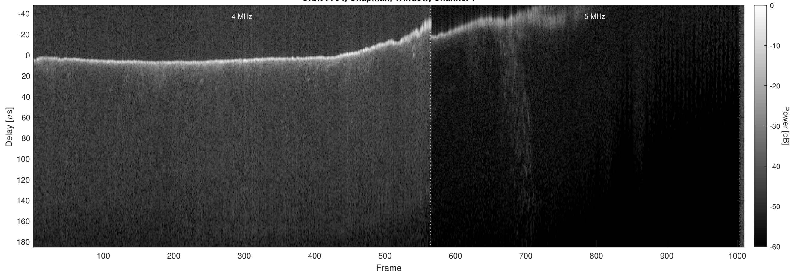
Orbit 7794, Chapman, Window, Channel 2
