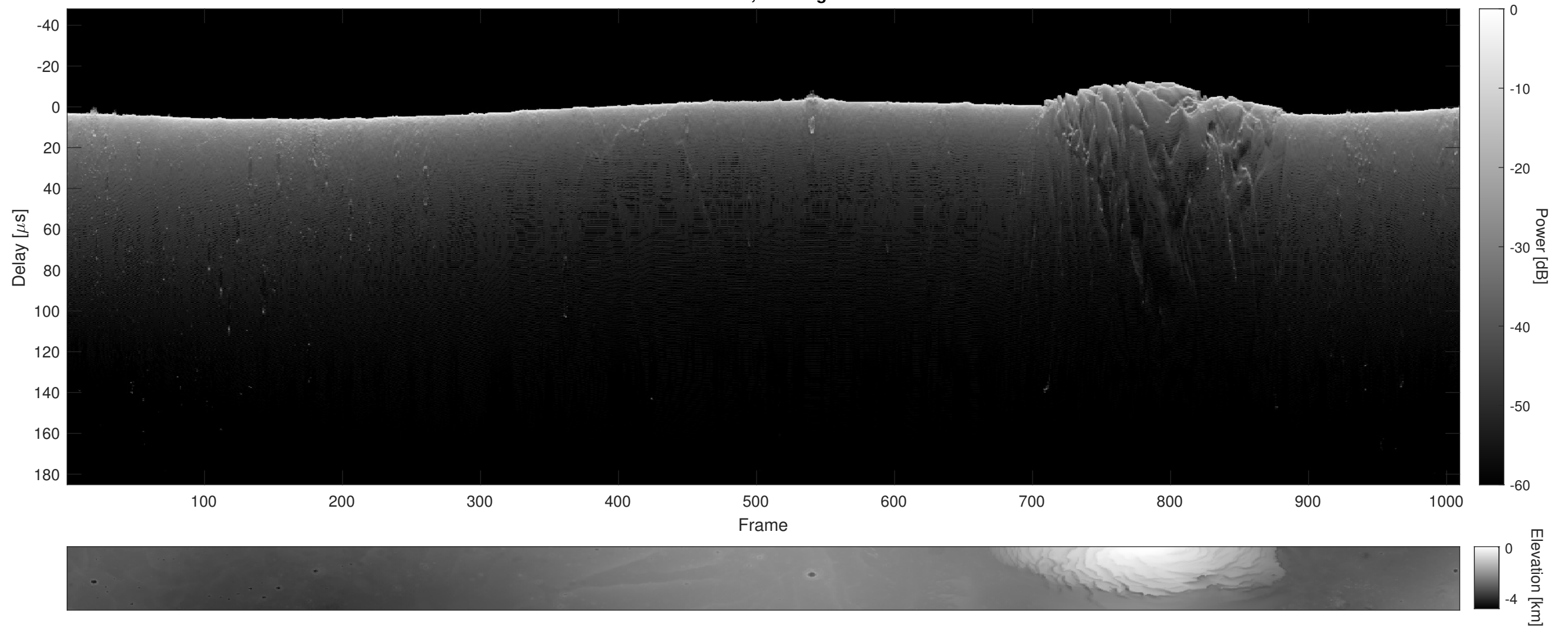
Orbit 7794, Cluttergram
