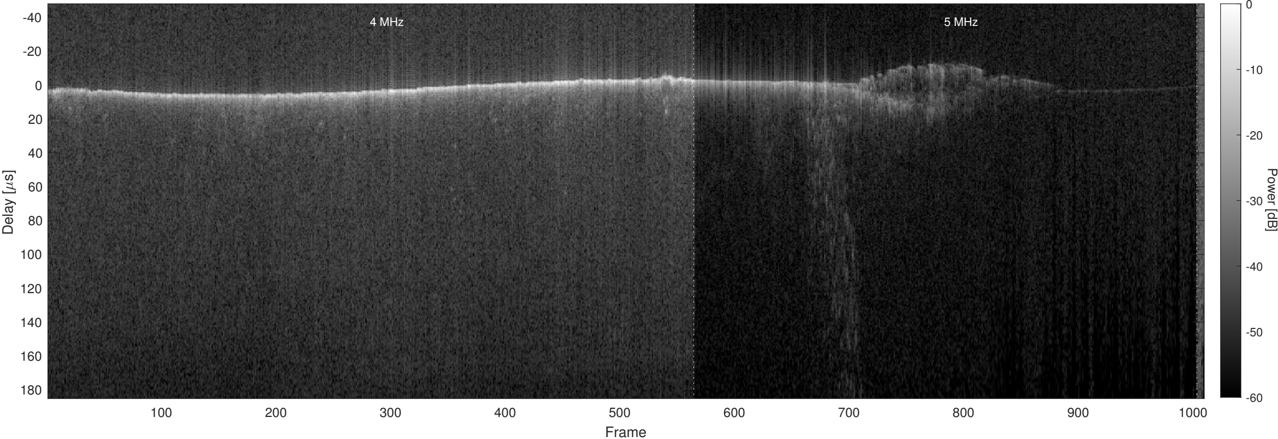
Orbit 7794, Optimized, No Window, Channel 2
