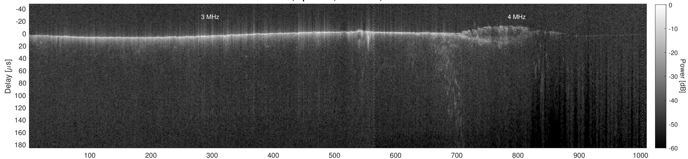
Orbit 7794, Cluttergram
