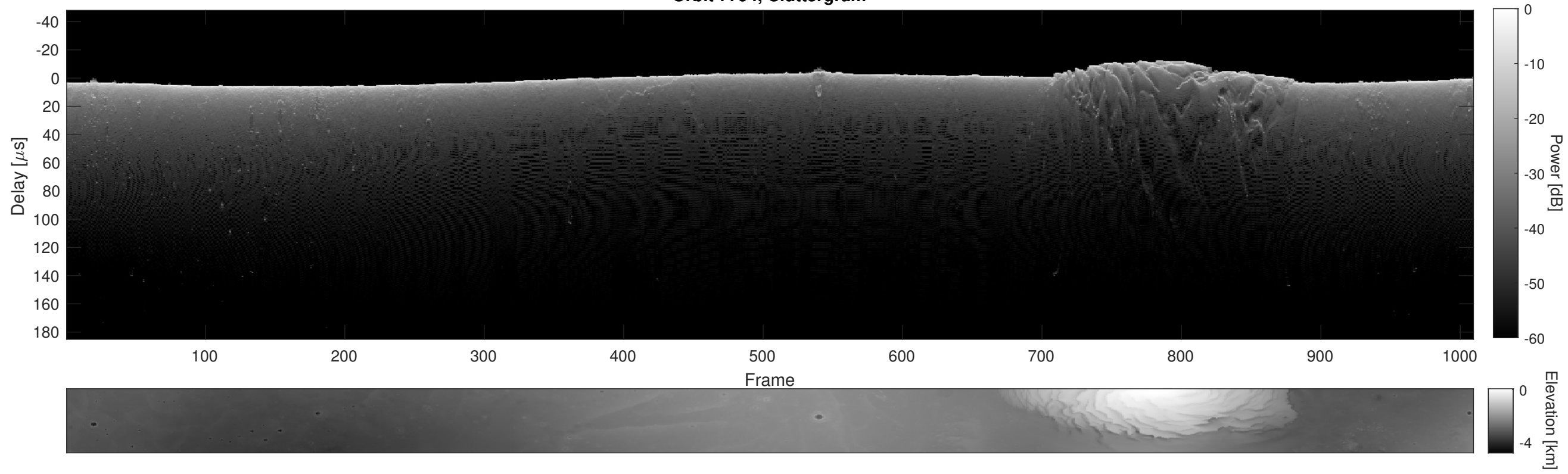
Orbit 7794, Cluttergram
