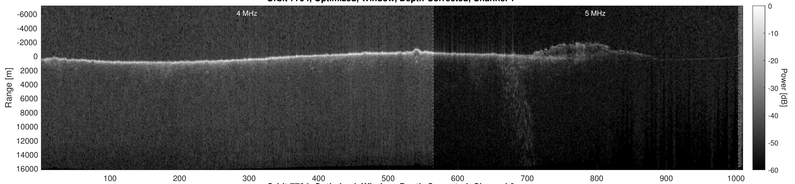
Orbit 7794, Optimized, Window, Depth-Corrected, Channel 2
