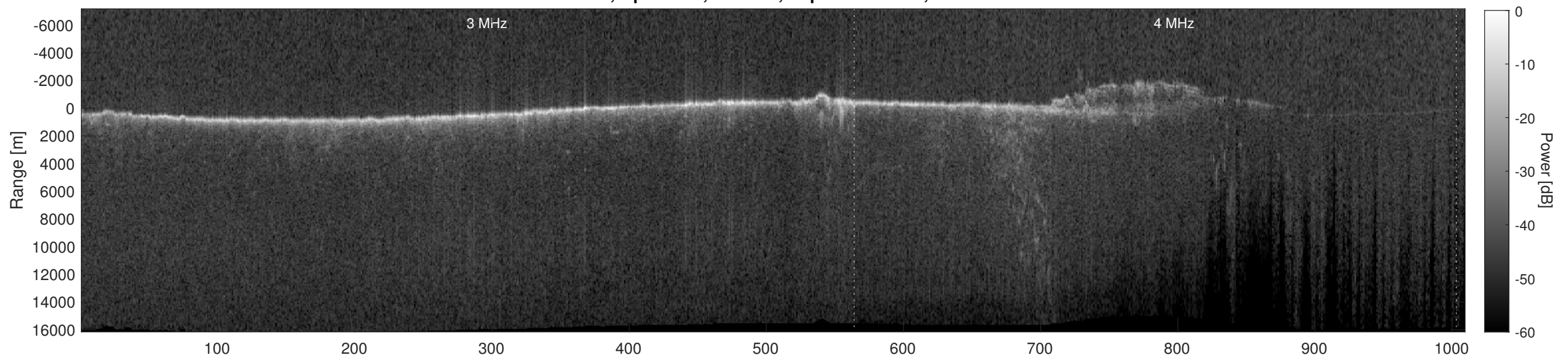
Orbit 7794, Depth-Corrected Cluttergram
