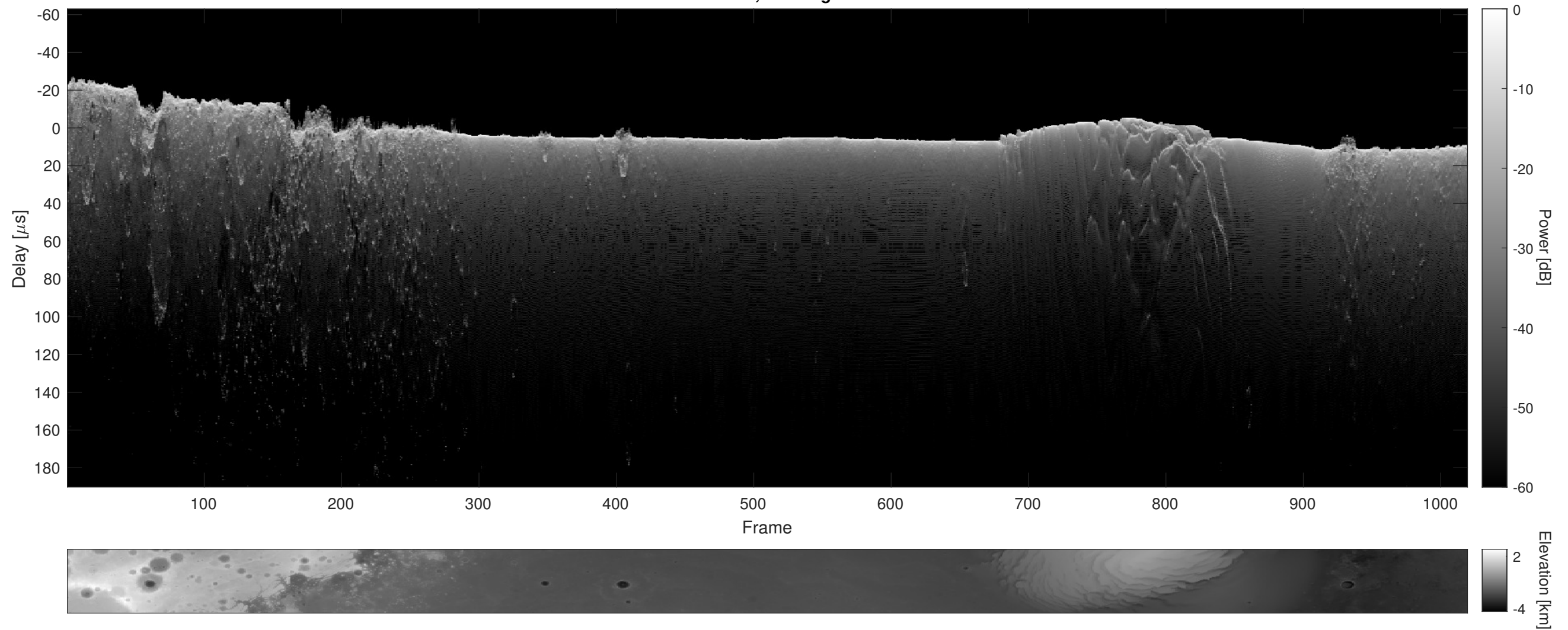
Orbit 7798, Cluttergram
