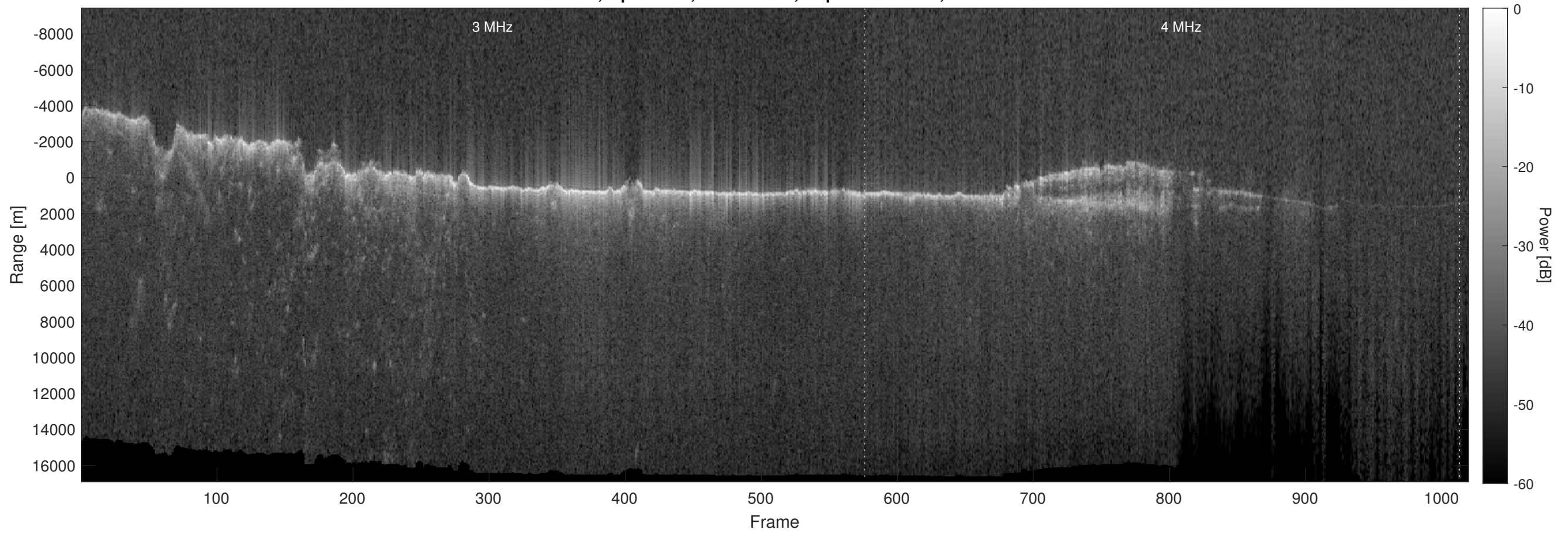
Orbit 7798, Optimized, No Window, Depth-Corrected, Channel 2
