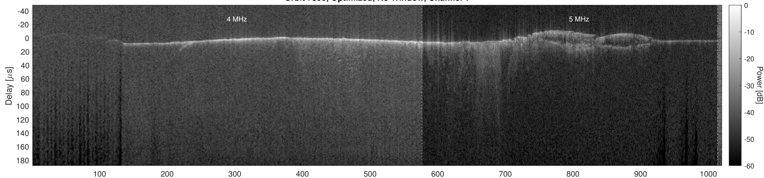
Orbit 7800, Optimized, No Window, Channel 2
