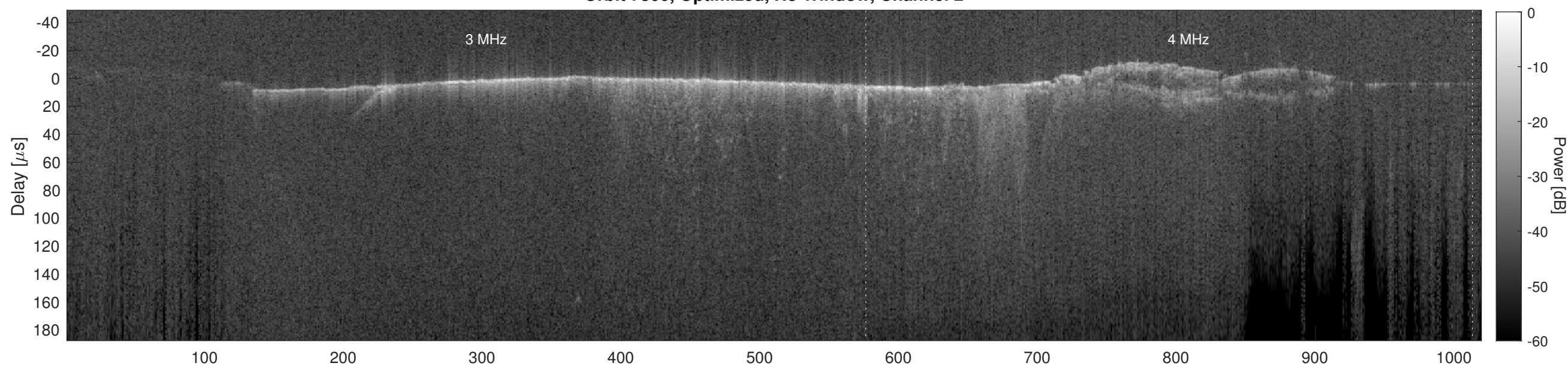
Orbit 7800, Cluttergram
