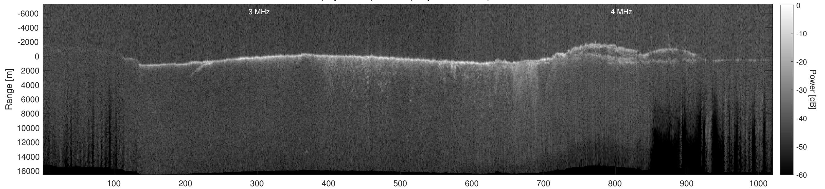
Orbit 7800, Depth-Corrected Cluttergram
