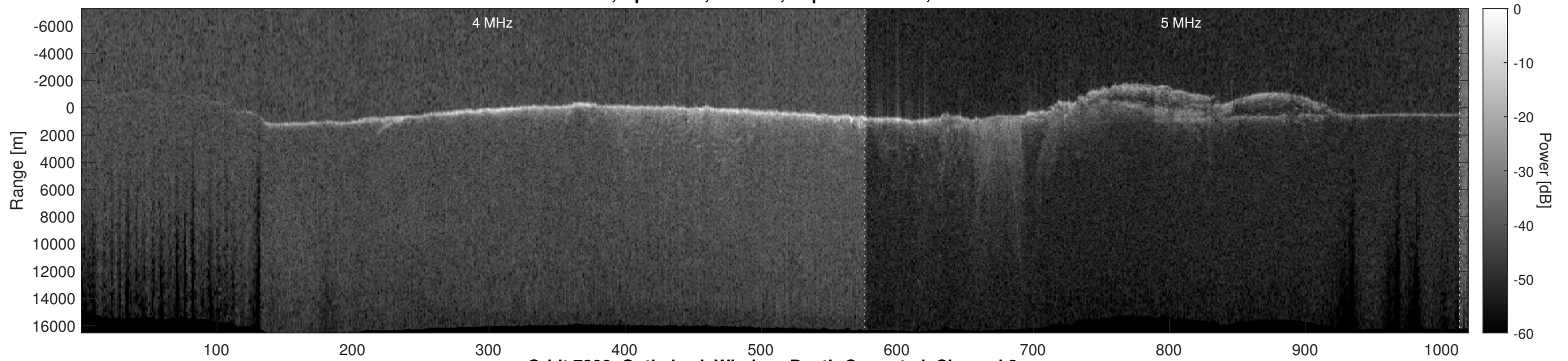
Orbit 7800, Optimized, Window, Depth-Corrected, Channel 2
