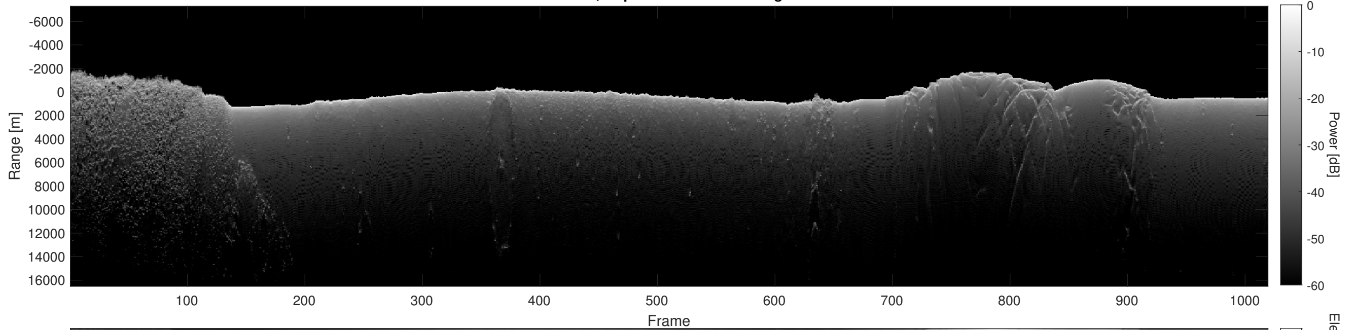
Orbit 7800, Depth-Corrected Cluttergram
