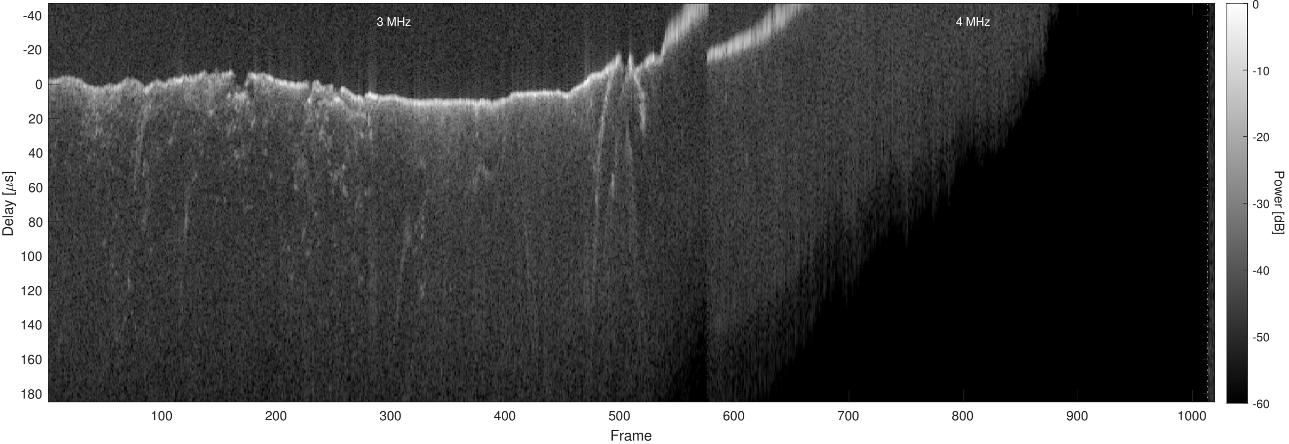
Orbit 7802, Chapman, Window, Channel 2
