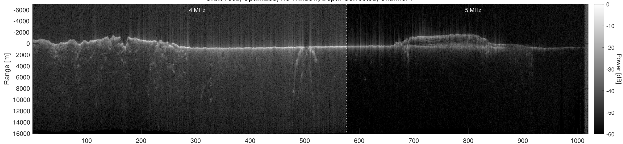
Orbit 7802, Optimized, No Window, Depth-Corrected, Channel 2
