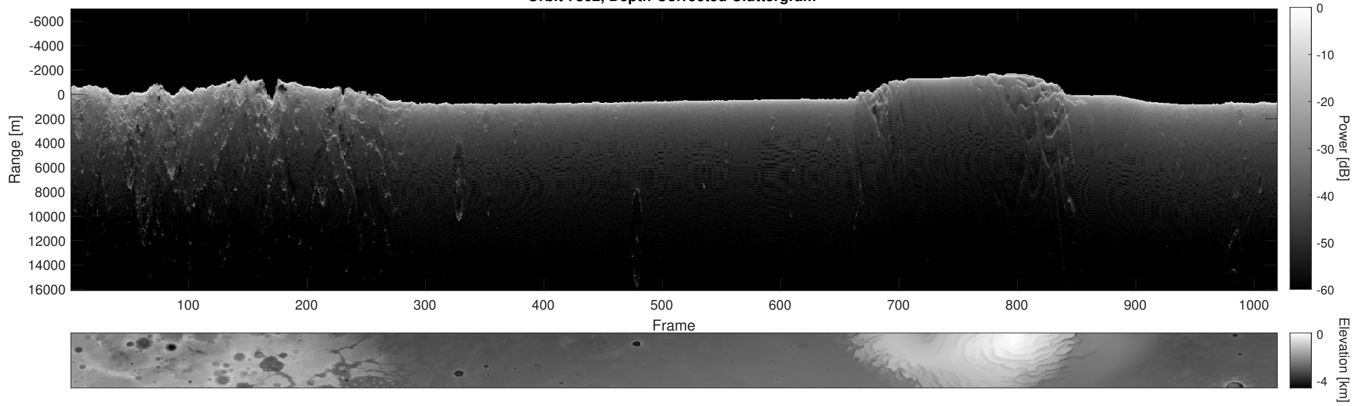
Orbit 7802, Depth-Corrected Cluttergram
